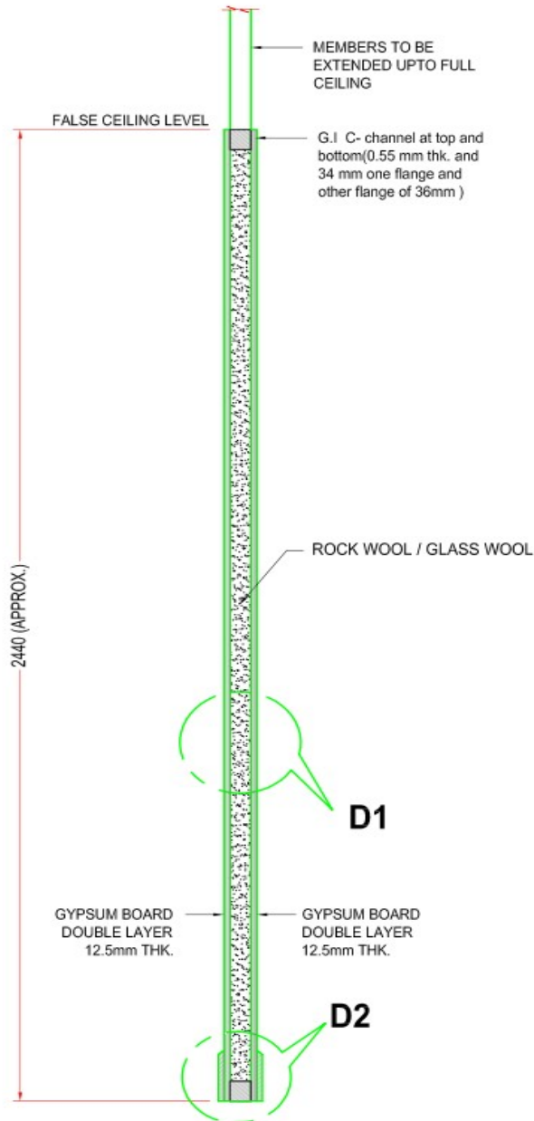
SECTIONAL SIDE VIEW
